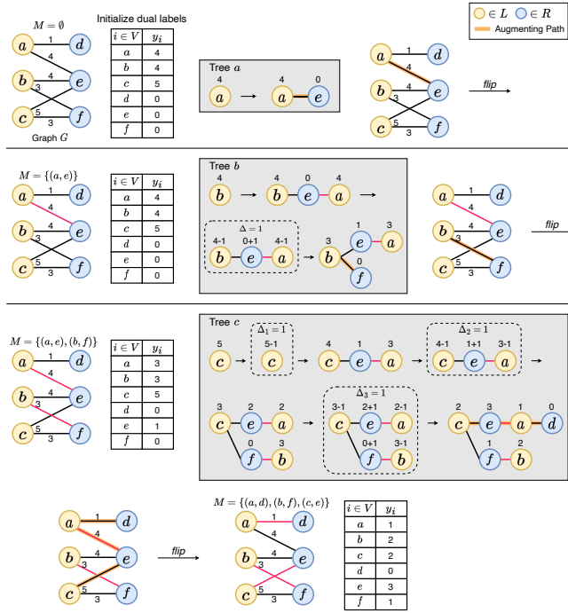
Figure 4: The execution pattern of the Hungarian algorithm on a graph G . Each row shows one search iteration. Dual label values are shown above vertices in the current search tree.
