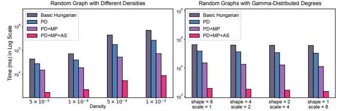
Figure 14: Effectiveness of phase decoupling (PD), multi-path batching (MP), and adaptive search (AS) under different densities and degree skews in random graphs with |V|=200,000
