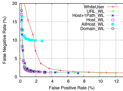
(a) Comparing different types of whitelists, varying the edge-weight-sum threshold
