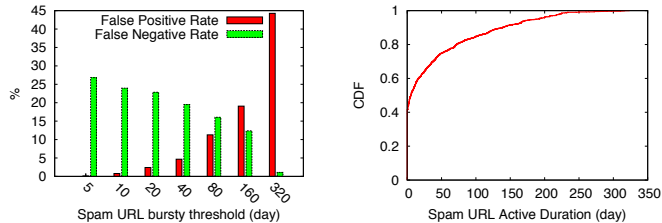
(a) AutoRE performance (b) Active duration of spam URLs
