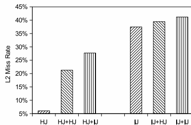
Figure 1: L2 miss rates when running a single or co-running various combinations of a hash join (HJ) and an index join (IJ).
